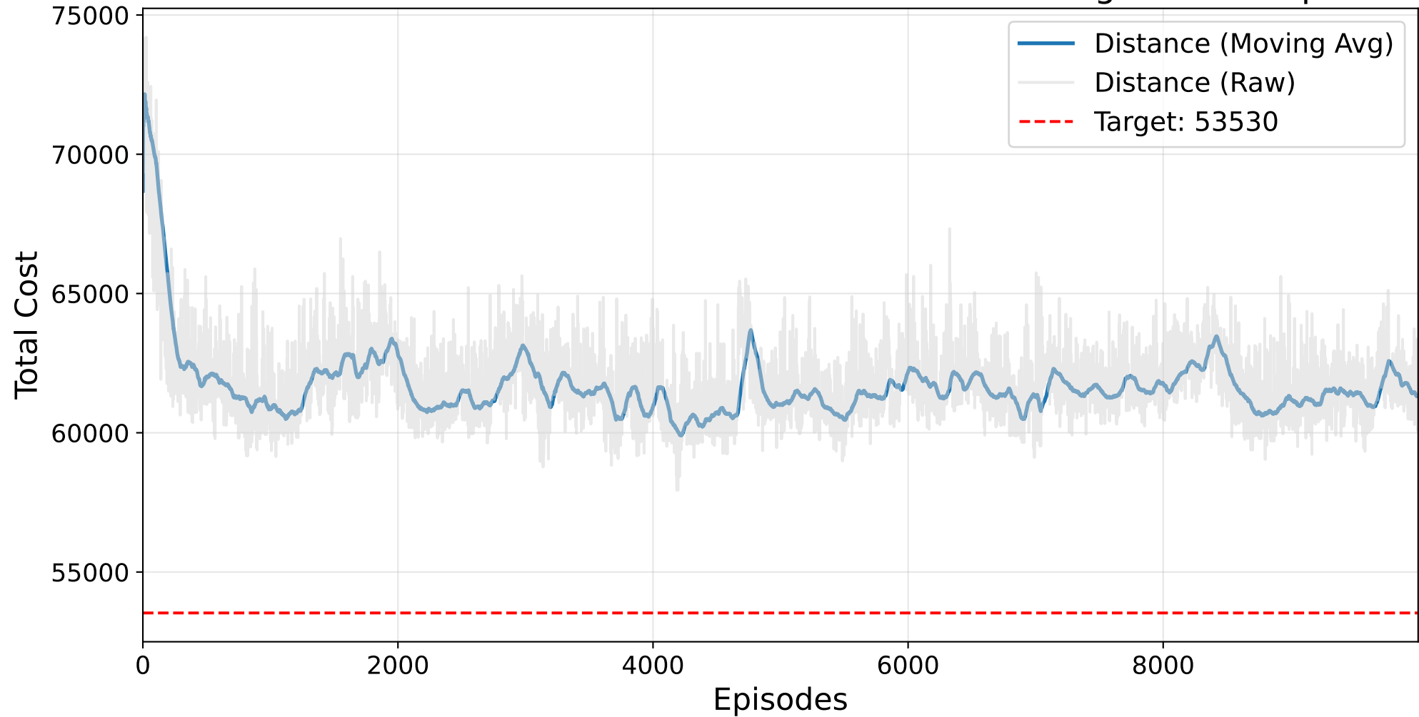
Final HYPERBAND TPE Masked AutoRL-SOP Training - ft70.4.sop
